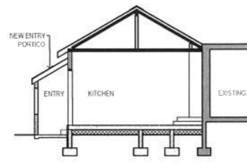
5 SECTION AA 1:100
