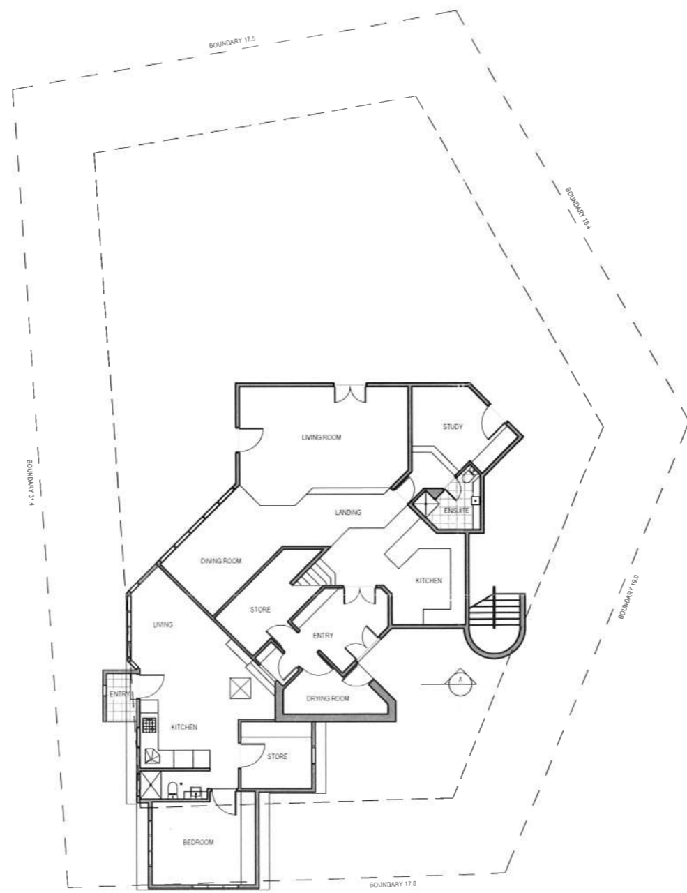
7 GROUND FLOOR 1:100
